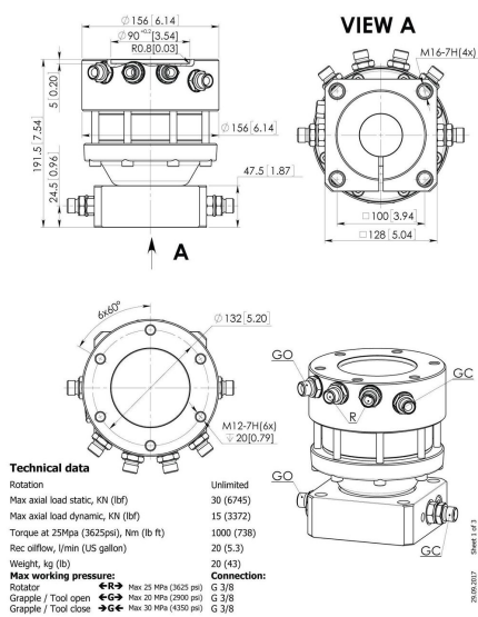
ROTATOR GR30FF
